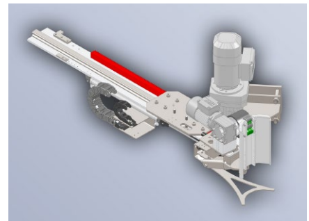
» Stretch-arm with rack drive
